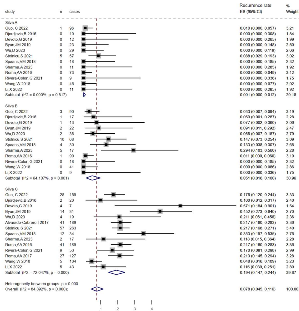
Figure S3. Forest plots of stratified Meta-Analysis of the recurrence rate of HPV-related endocervical adenocarcinoma. Thirteen studies [5,6,12,17-21,25-28,32] reported the relationship between Silva A, B, C and recurrence, while one study [24] reported the recurrence rate of 189 patients with Silva C.
